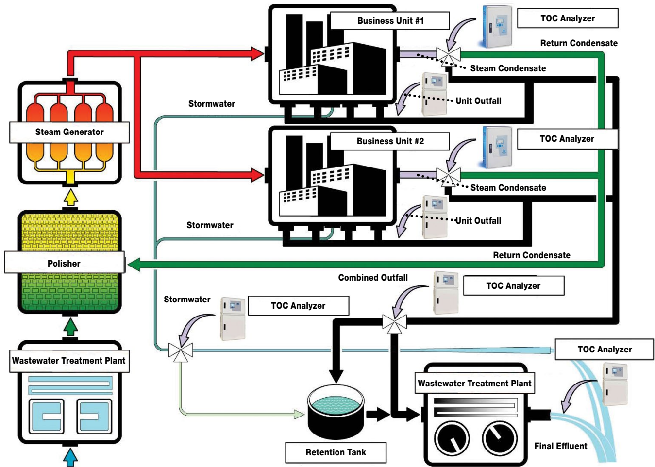
Figure 4: Summary of TOC Chemical and Petrochemical Applications
