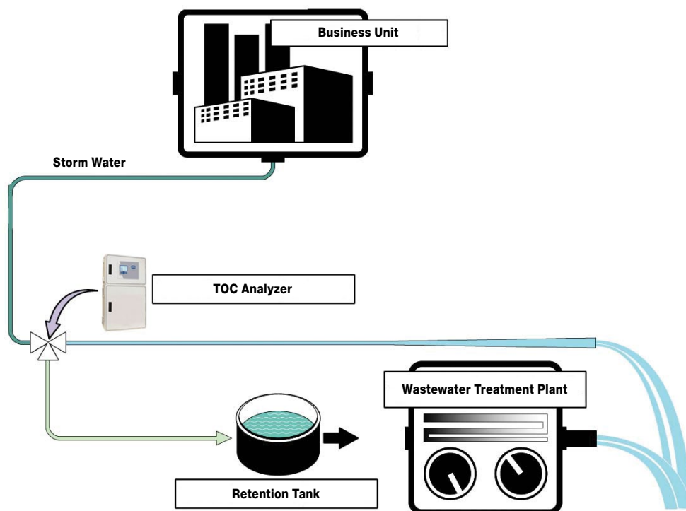
Figure 2: TOC stormwater application
