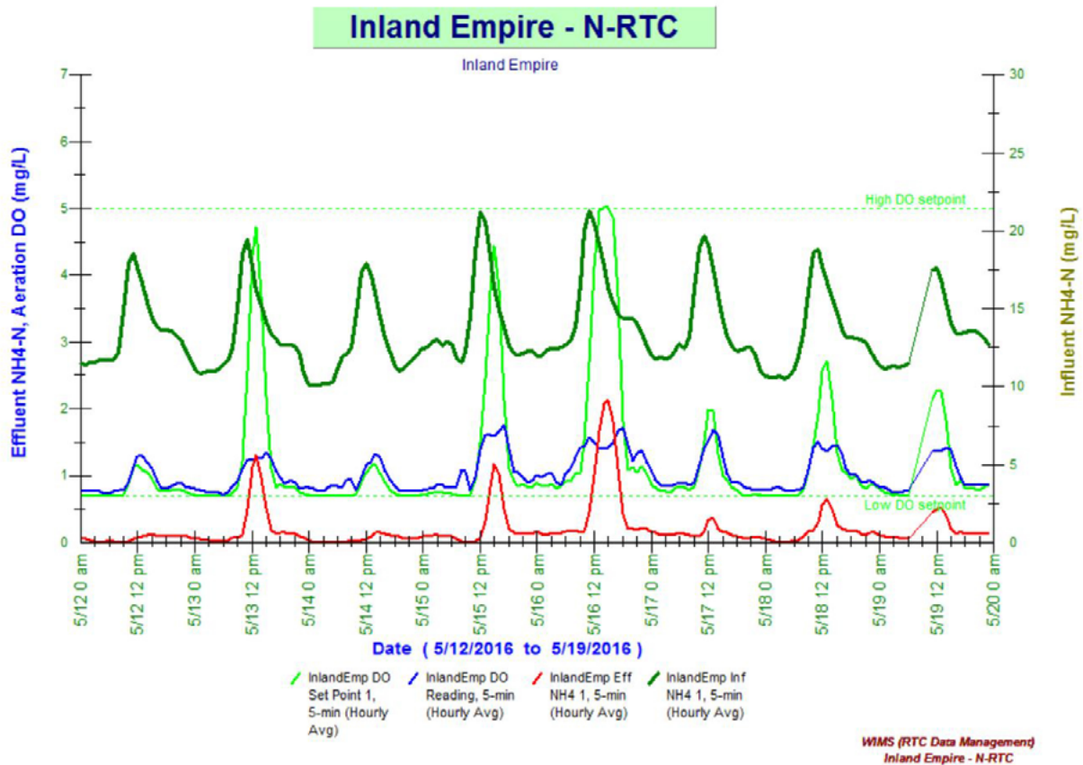
Figure 3: RTC-N DO and ammonia readings
